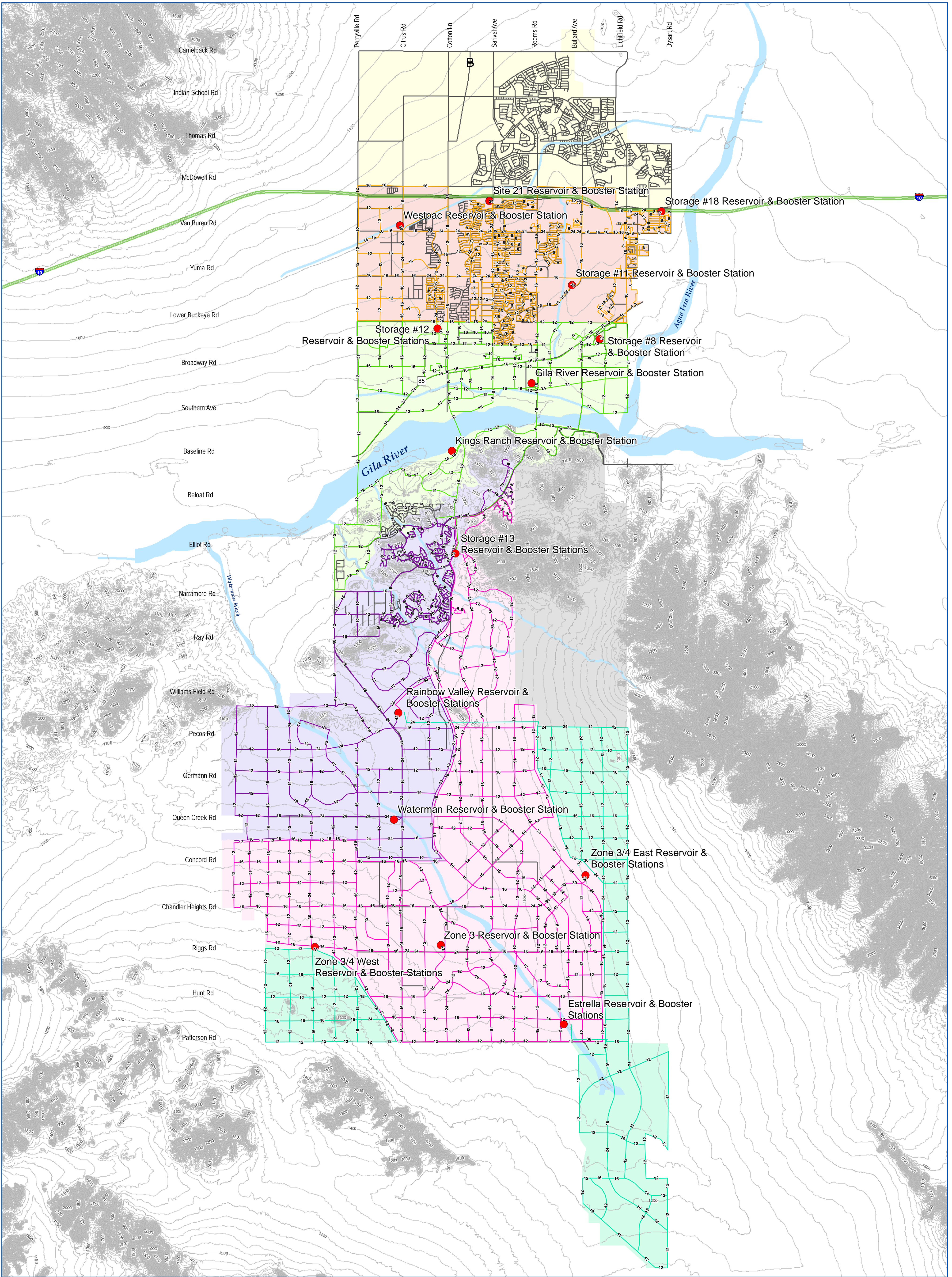
Figure 11 Build Out Water Distribution System Integrated Water Master Plan City of Goodyear, AZ 2007
